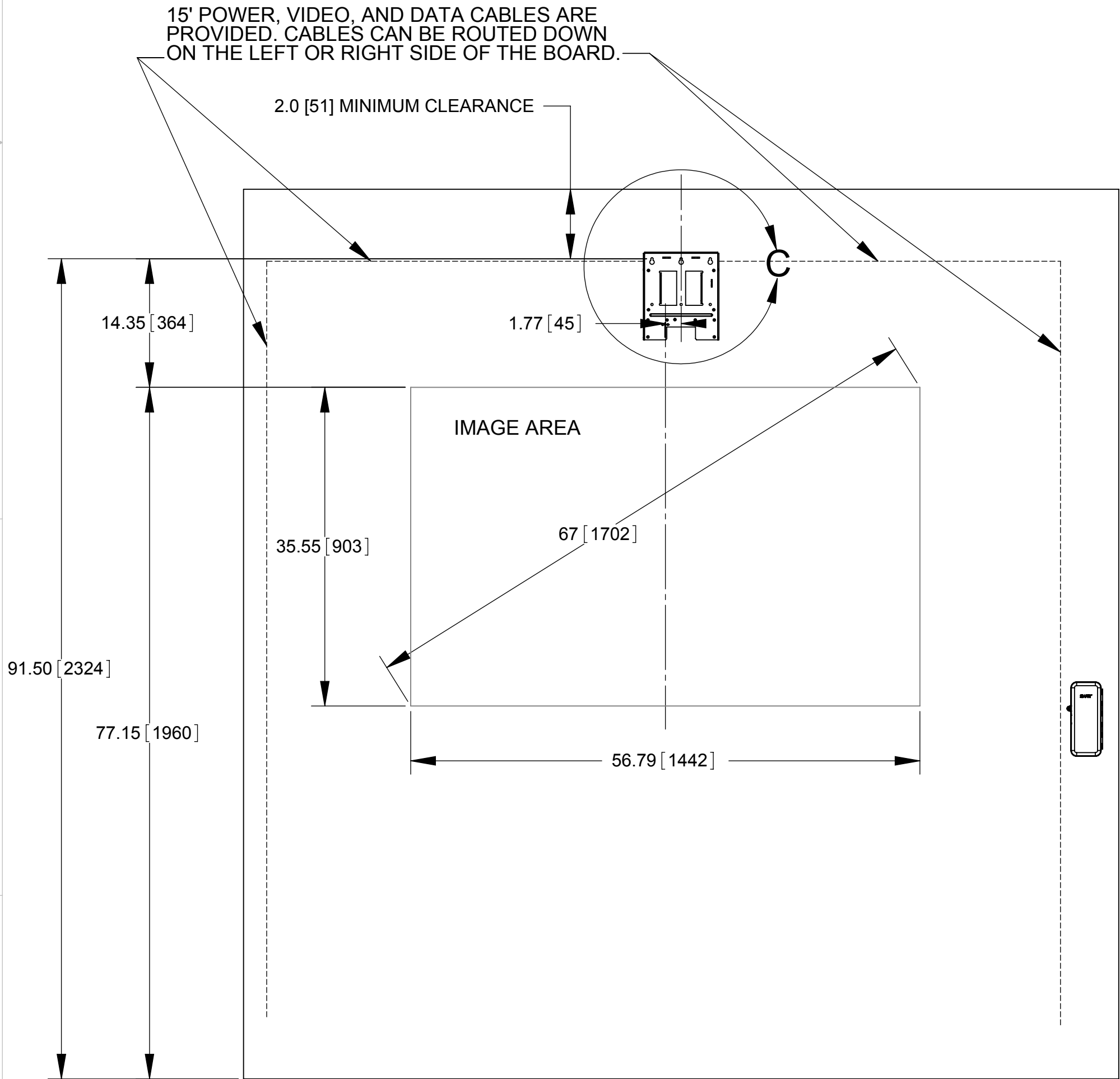
67" (Minimum Image Size) Front View
