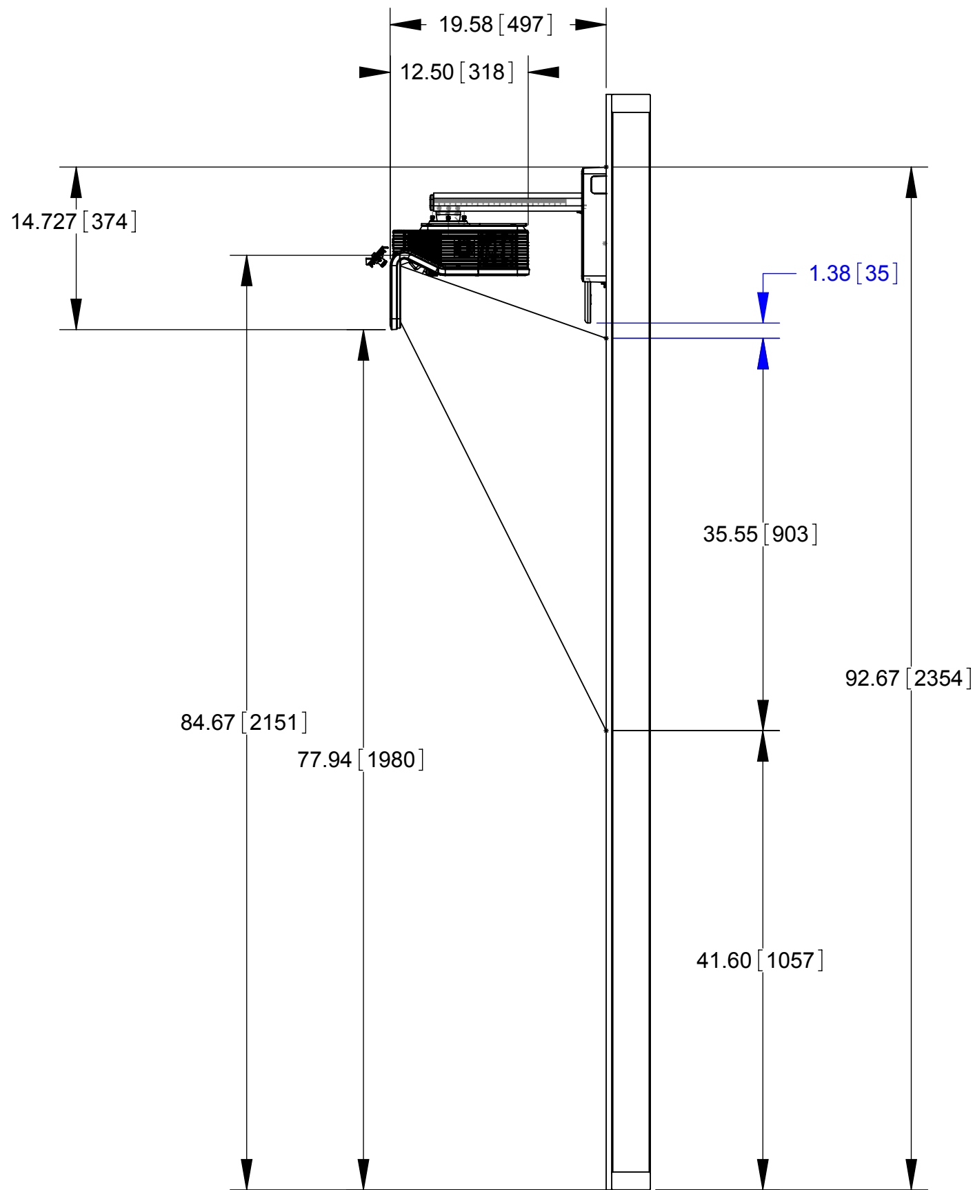
67" (Minimum Image Size) Side View
