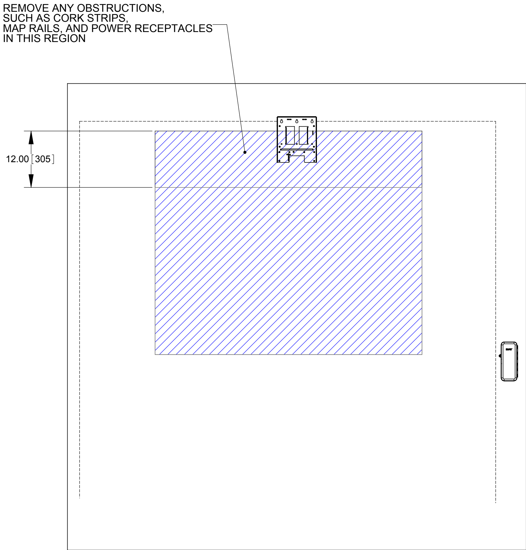
67" (Minimum Image Size) Front View
